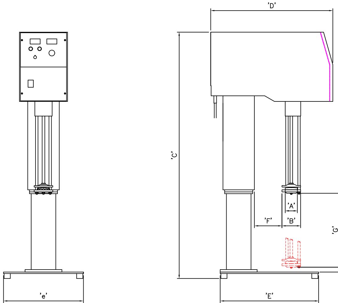
MIXER DIMENSIONS – DISTROMIX BATCH LABORATORY SERIES – ELECTRIC LIFT MODELS
